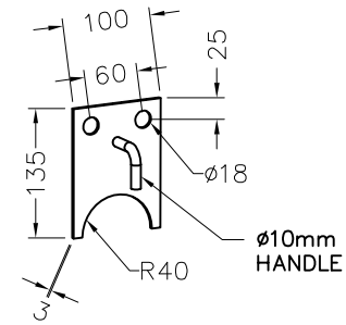
CHUTE COVER DETAILS (SUPPLIED ON REQUEST)
