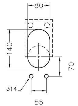
OPERATOR & FAR SIDE MOUNT HOLES & CUT-OUT DETAILS - BY OTHERS
